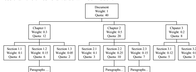
Figure 1. An Example of Fractal Summarization Model
